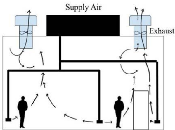
FIGURE 2. DISPLACEMENT VENTILATION
