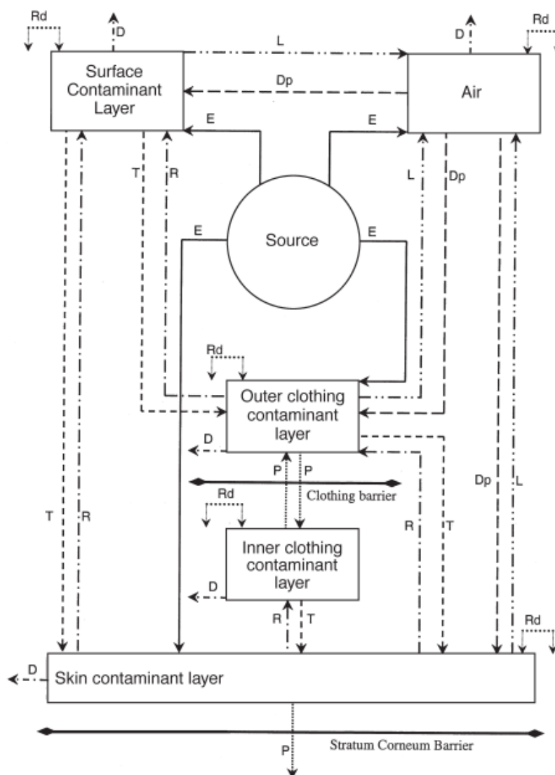
Fig. 1. The conceptual model. Adapted from Schneider et al. (1999). Overview of the conceptual model, compartments and transport processes. (E=Emission (—), Dp=Deposition (---), L=Resuspension/Evaporation (···), T=Transfer (- · -), R=Removal (---), Rd=Redistribution (· · ·), D=Decontamination (- · - ·), P=Penetration/Permeation (····)).
